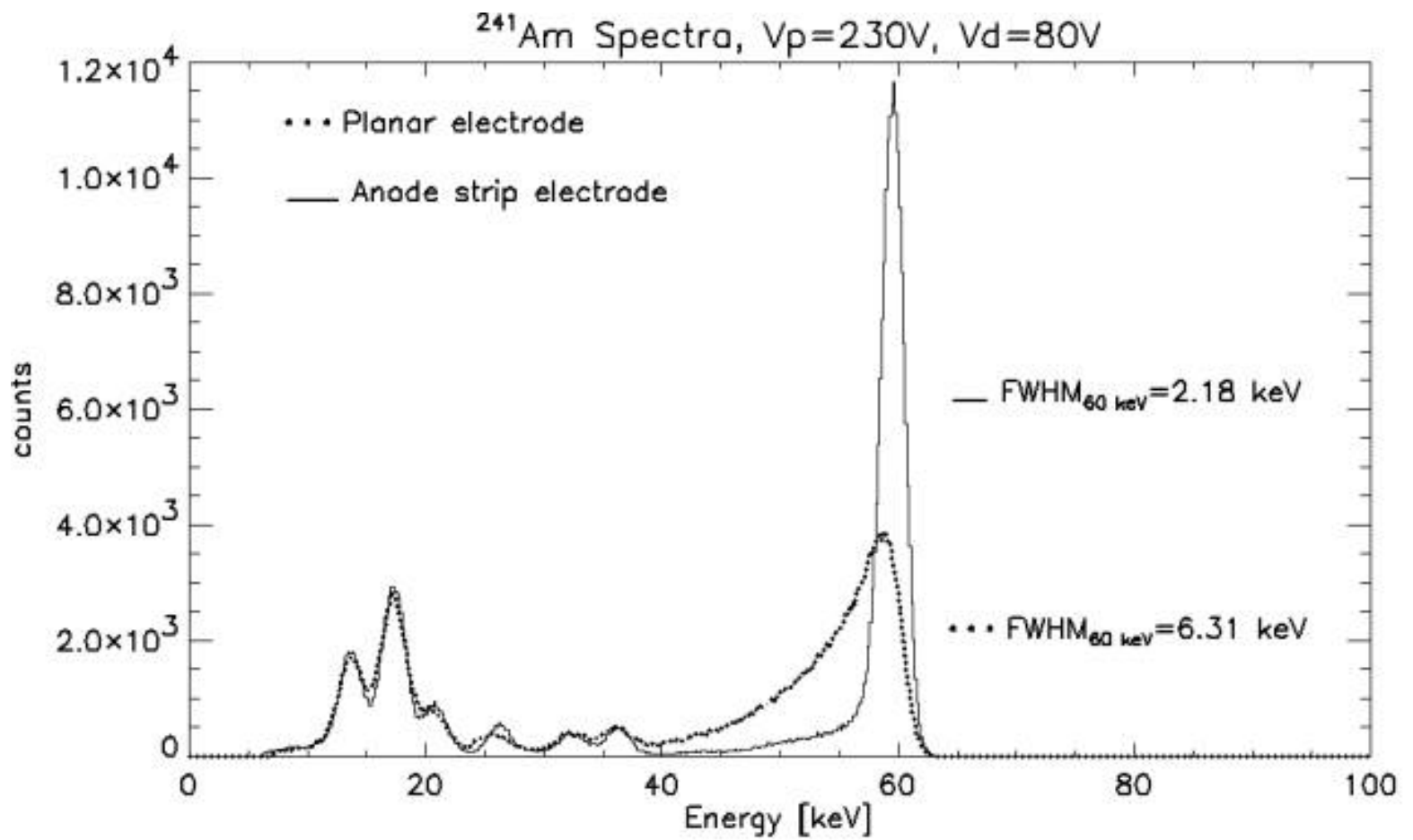
Figure 2. ^{241}\text{Am} spectra obtained with the planar electrode (dotted line) and the anode strip (full line).
