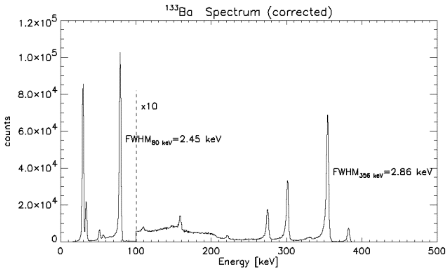
Figure 4. 133 Ba spectrum corrected for hole trapping (see text). The spectrum is multiplied by 10 above 110 keV.
