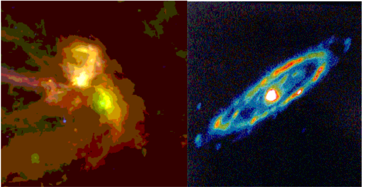
Figure 1. Examples of the legacy of IRAS. (Left) The Rho Ophiuchi star forming region and (Right) M31. In the images the colors blue, green, and red correspond to 12, 60, and 100 \mu\text{m} , respectively.
