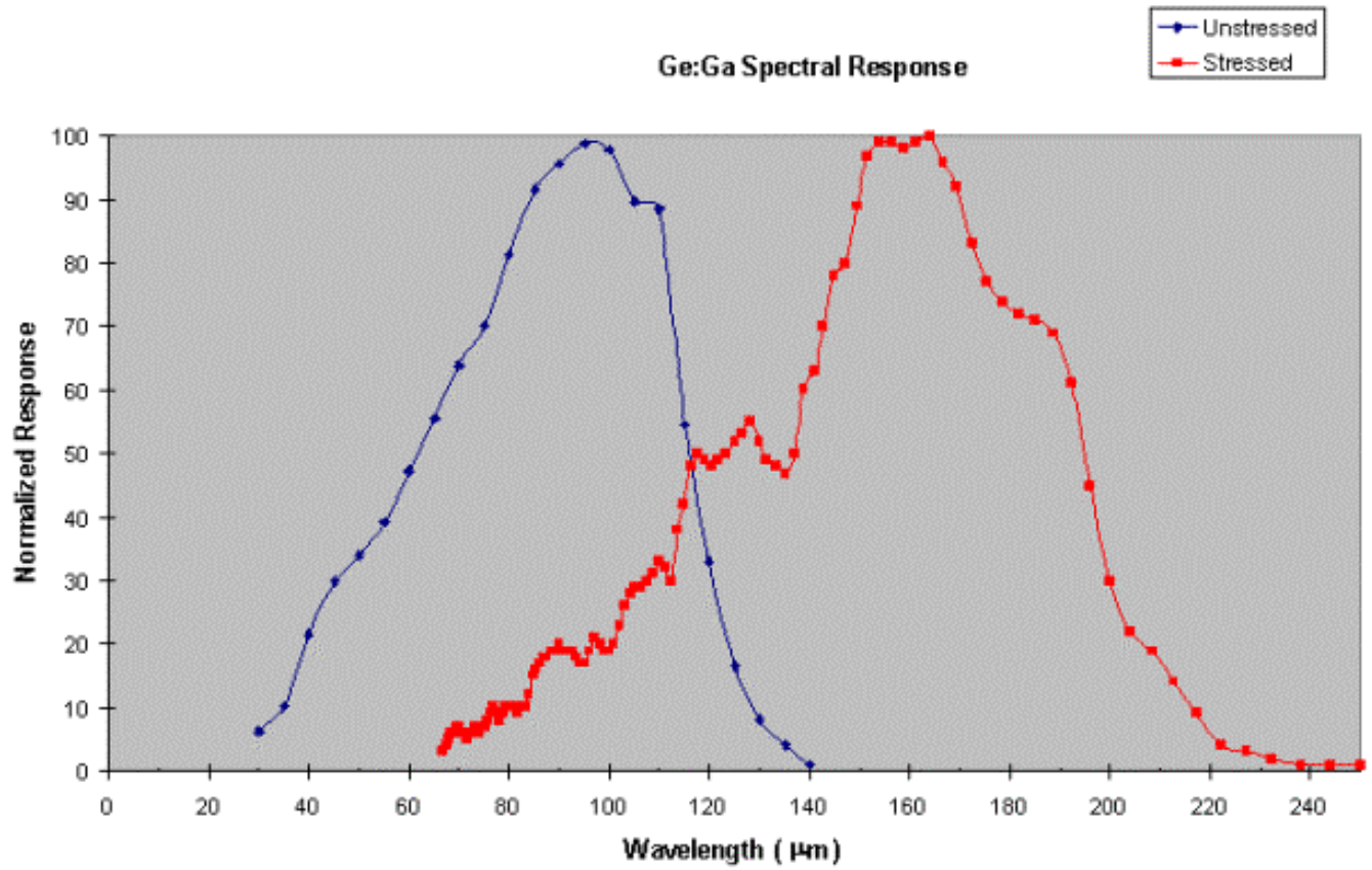
Figure 2. Spectral Response for Stressed and Unstressed Ge:Ga.
