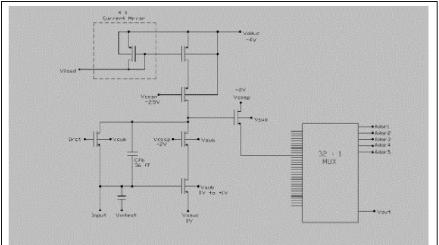
Figure 3. Circuit Diagram for CRC-696 CTIA Multiplexer
