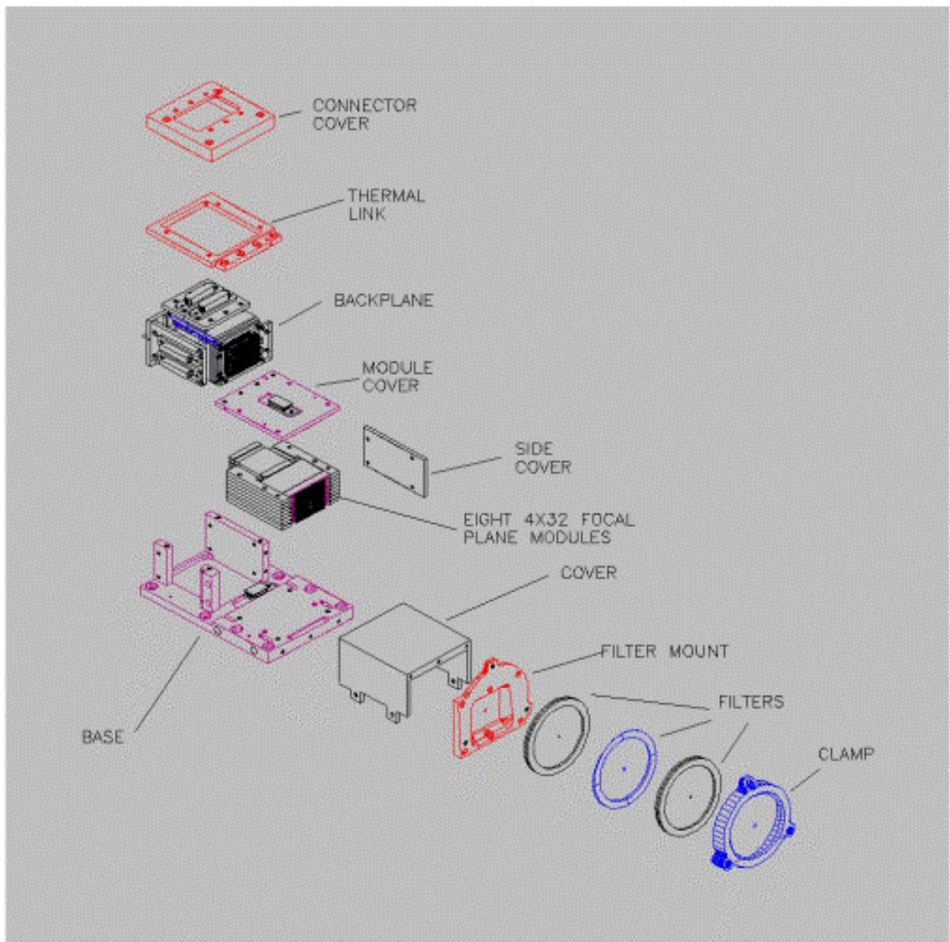
Figure 4. Major components of the MIPS 70 μm Array.
