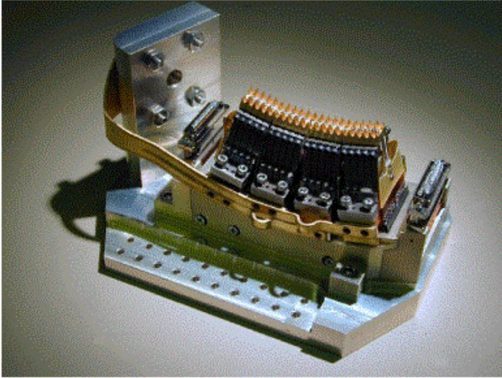
Figure 6. MIPS 160 \mu\text{m} Stressed Ge:Ga Array
