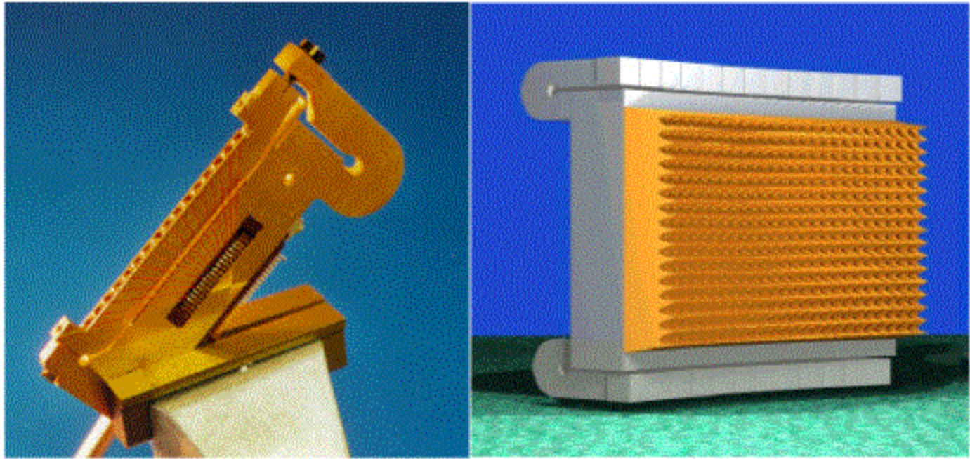
Figure 9. (left) FIFI-LS Stressed Array Module. (right) CAD Model of Full FIFI-LS Stressed Detector Array (A. Poglitsch)
