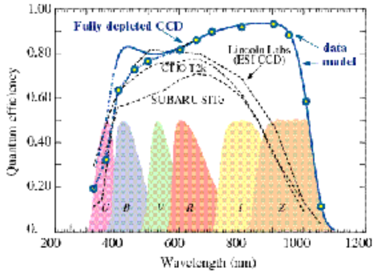
Figure 2. Measured response of the fully-depleted CCD at 100 °C (open circles) for an unoptimized two-layer AR coating (the dark curve through the points is a model calculation). Response is expected to be significantly higher for optimized AR coatings. For comparison, measured response of the 2k x 4k deep-depletion back-illuminated MIT/Lincoln chip on Keck ESI is shown, as are measurements for two different S110 CCD's on SUBARU and CTIO. Relative spectral responses of standard wide-band filters are shown.
