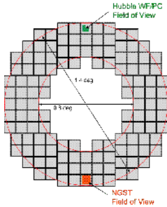
Figure 4. The 1° x 1° imager focal plane populated with 128 3k x 3k, 10.5 mm 2 CCD's.
