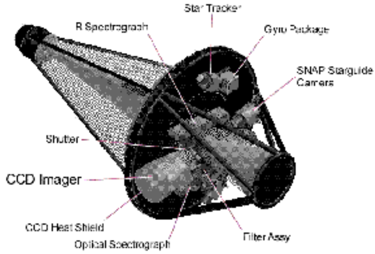
Figure 5. Conceptual satellite optics design for a three mirror anastigmat telescope showing the position of the CCD imager at the focal plane.
