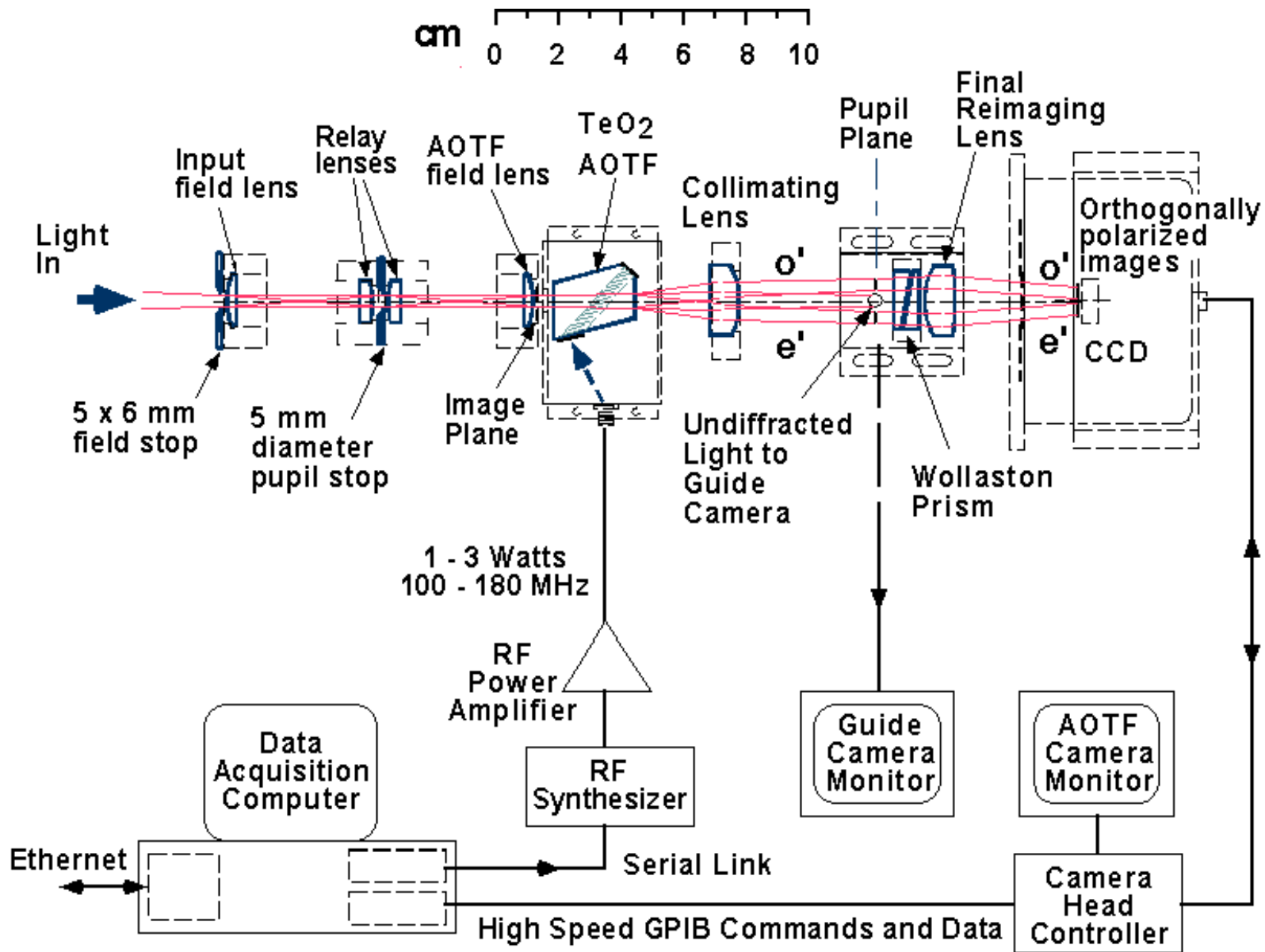
Fig. 1 – Optical design of the AOTF Camera and block diagram of the data acquisition setup used at the Starfire Optical Range, 1.5-m Laser Beacon Facility.
