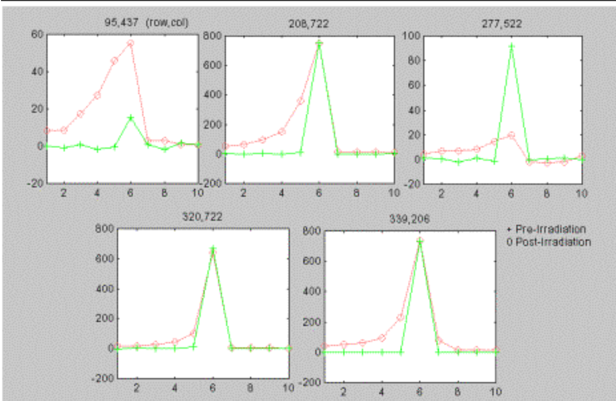
Figure 1 Example of Vertical Traces Around Defect Pixels Before and After Irradiation. Background Subtracted using 1-D Highpass Butterworth Filter in Horizontal
