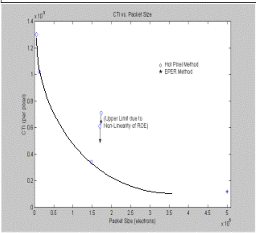
Figure 2 CTI vs. Packet Size for Irradiated CCD (this study)
