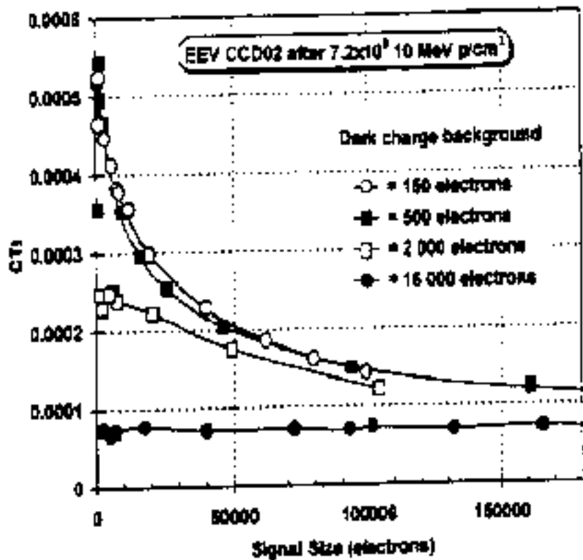
Figure 3 CTI vs. Packet Size and Background (spot illumination method). Reproduced from [7]
