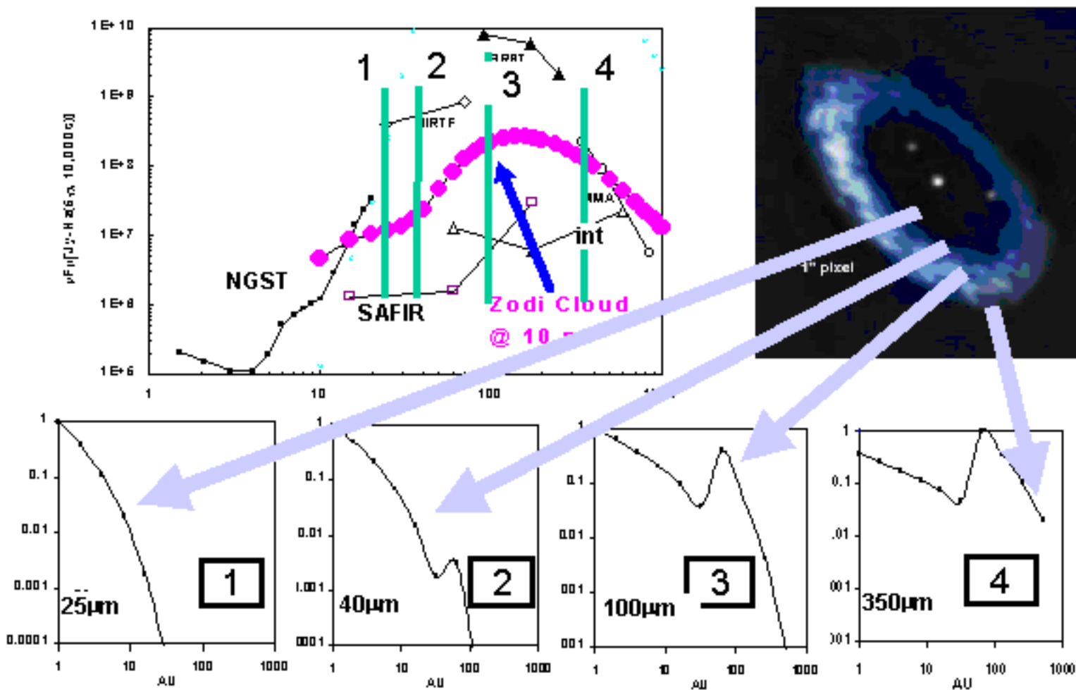
Figure 10. Images of debris disks at different wavelengths reveal different aspects of their structure.
