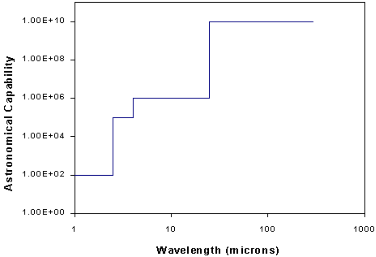
Figure 12. Gain in Astronomical Capability over the present with the advances discussed above.
