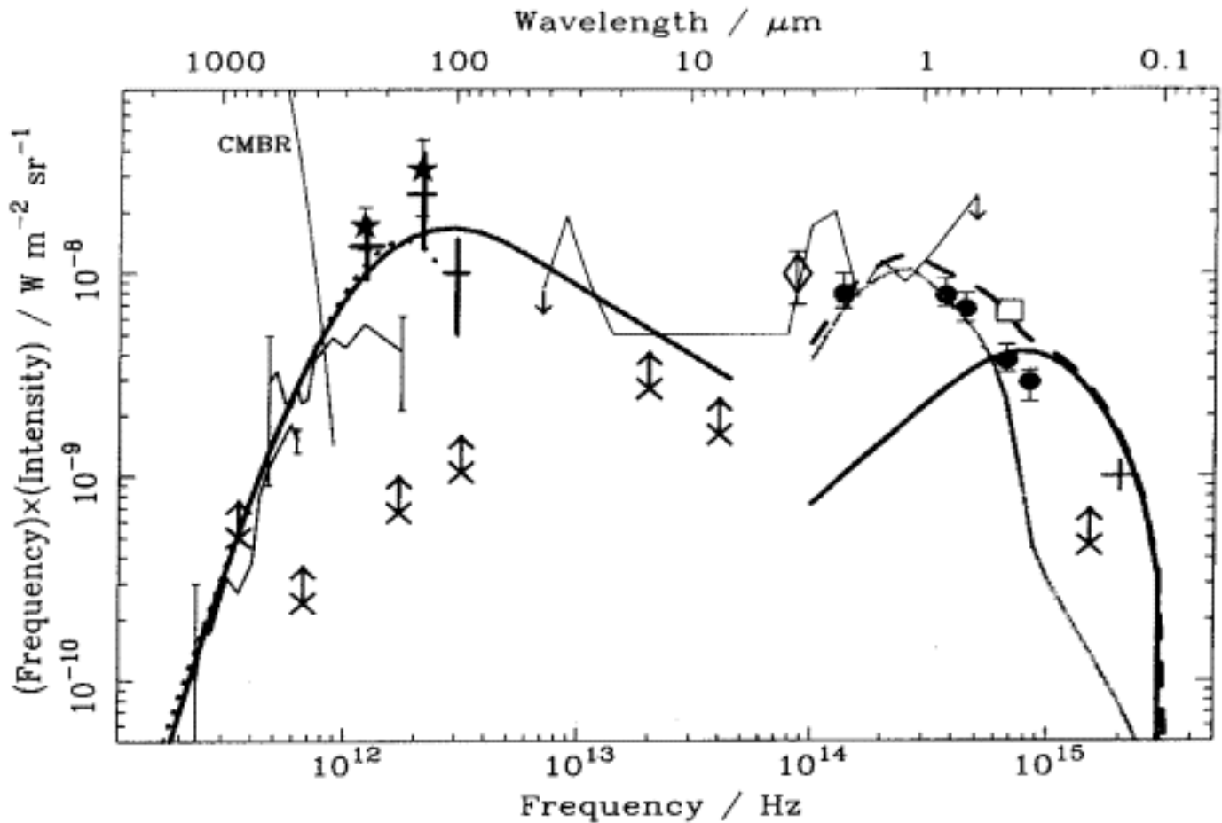
Figure 3. Cosmic energy density between 0.1 m m and 2mm wavelength. The various upward pointing arrows indicate counts of point sources, while the heavy solid and dashed lines show the results of large beam measurements and models that measure or predict the true absolute sky brightness. This plot and subsequent ones in the report are in \nu F_\nu or similar units, so a horizontal line represents constant energy per logarithmic frequency or wavelength interval.
