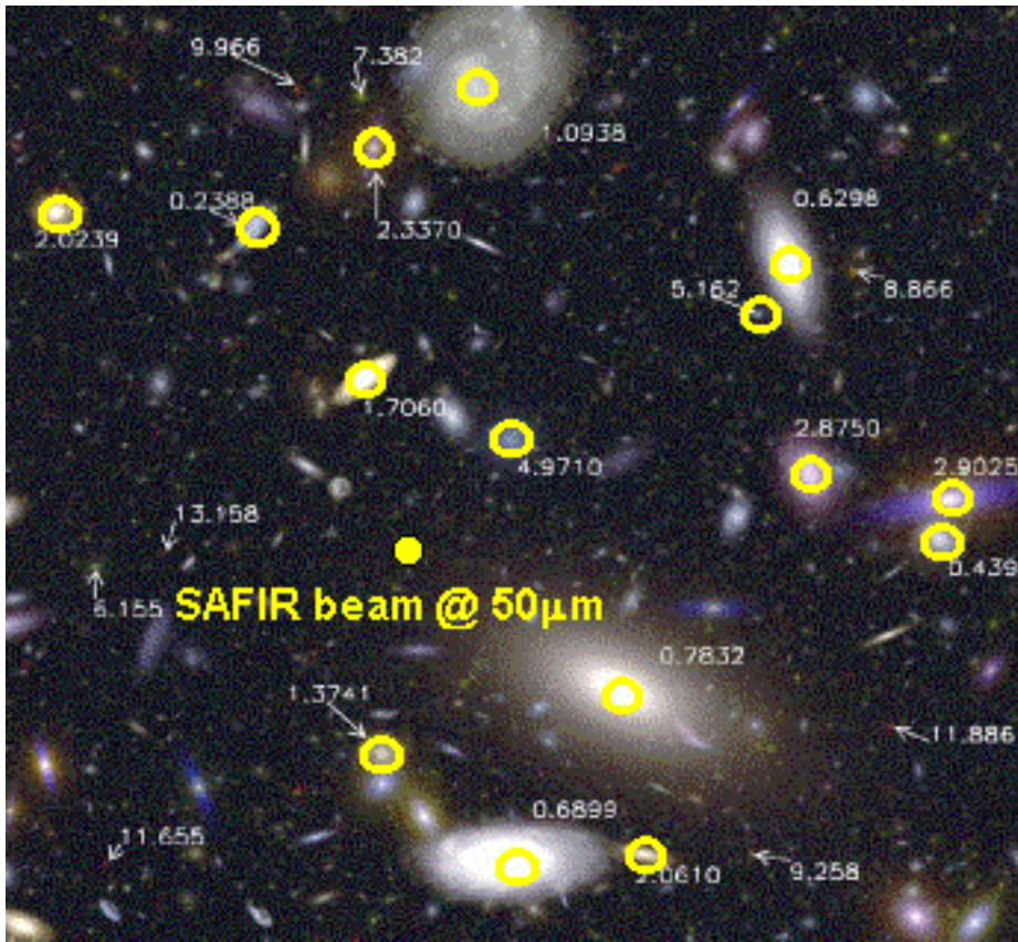
Figure 4. Simulated NGST deep field with 1'' beam of SAFIR placed on all labeled galaxies at z \leq 5 .
