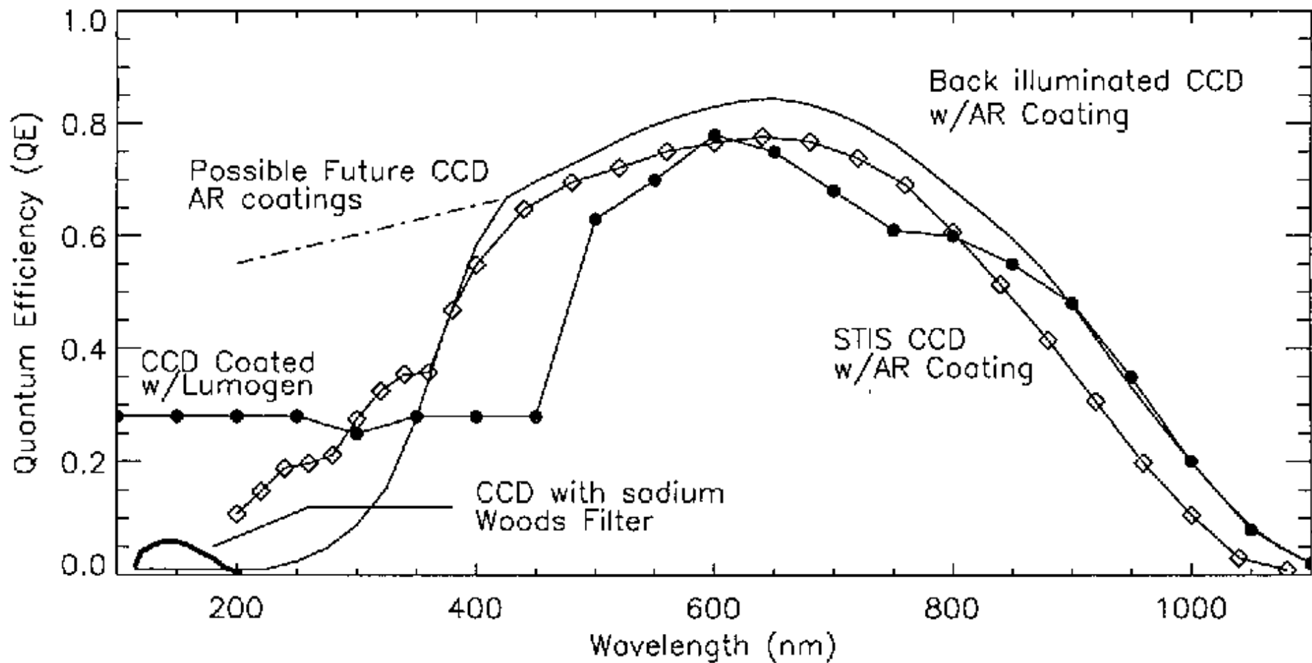
Fig. 3 showing QEs of various configurations of thinned back illuminate CCDs.
