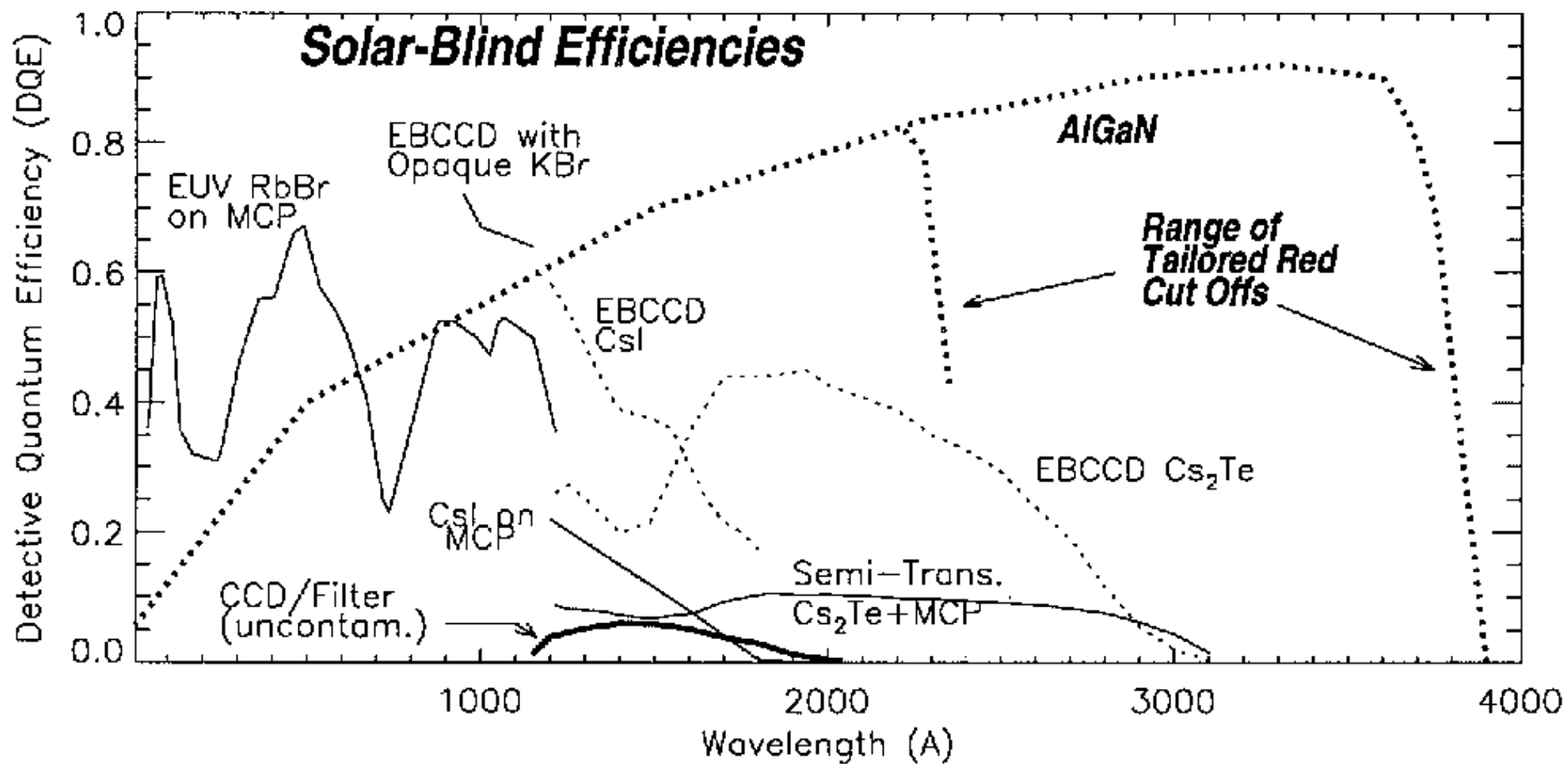
Fig. 4 showing solar-blind UV DQEs of various detectors.
