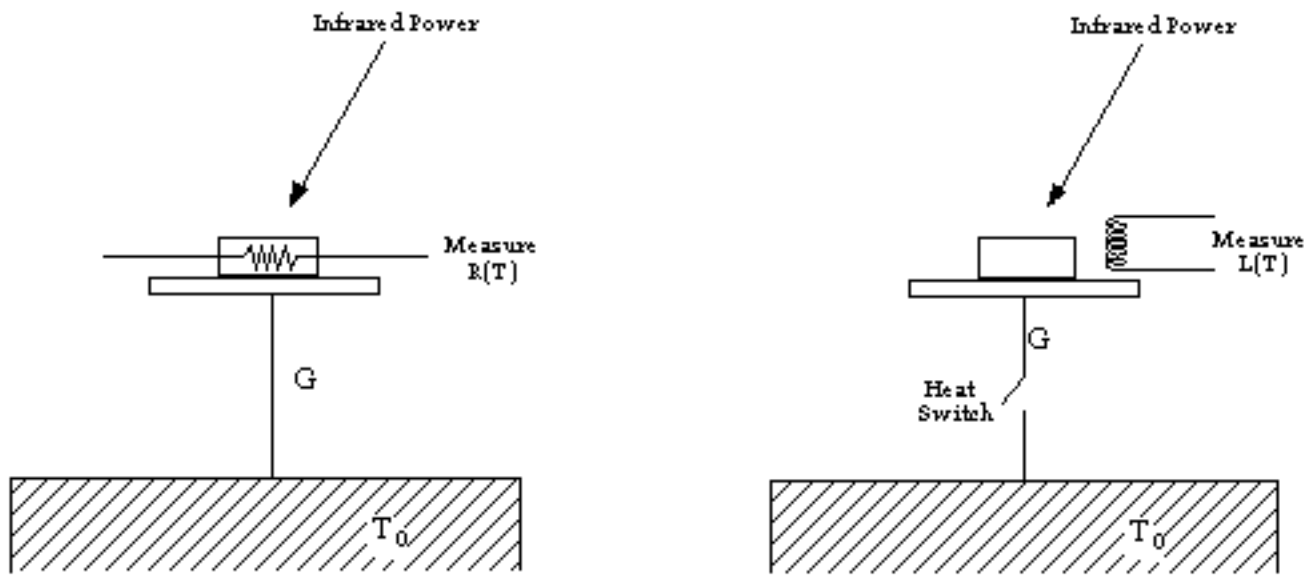
Fig 1: Schematic of resistive bolometer (left) and integrating bolometer (right). The integrating bolometer uses a heat switch and non-dissipative thermometer to provide greatly increased sensitivity and lossless integration.
