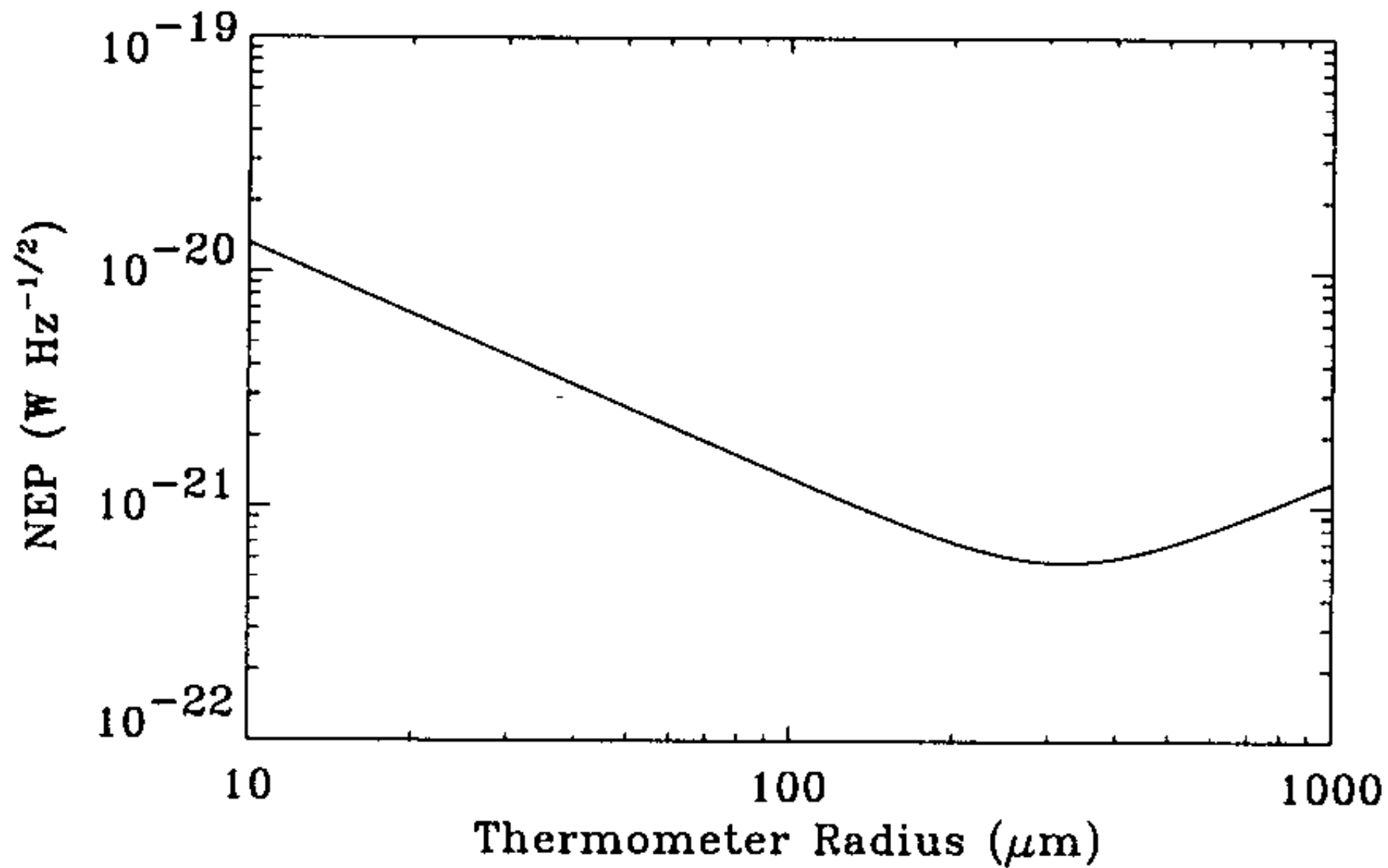
Fig 3: Predicted NEP vs sensor size for ideal integrating bolometer at 50 mK. Phonon noise dominates at small sizes, and SQUID noise for large sized. A heat switch period Dt = 0.1 ms is shown.
