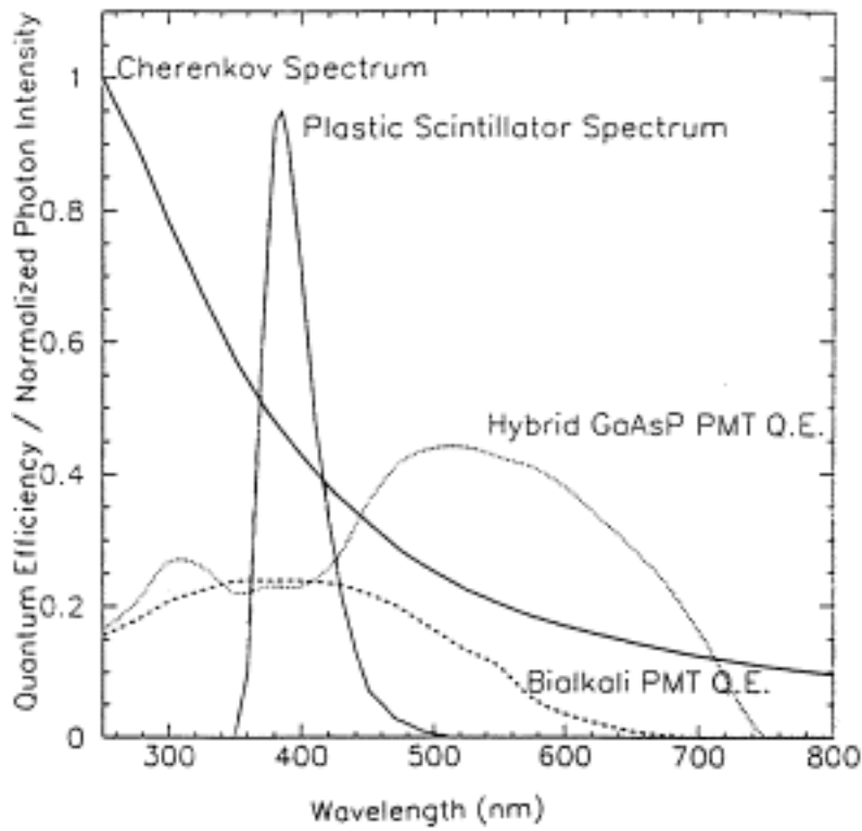
Figure 1. Quantum efficiency spectral dependence for two photomultiplier tubes shown along with Cherenkov radiation and plastic scintillator emission spectra.
