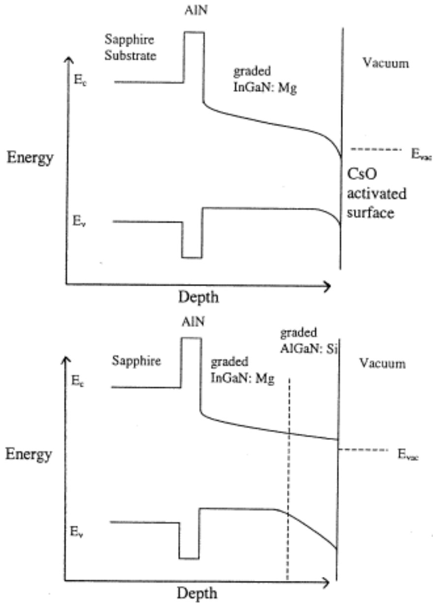
Figure 2. Spatial profiles of conduction and valence band edge energies, E_c and E_v respectively, for composition variations versus depth in two different photocathode heterostructures shown at the top and bottom. E_{vac} is the vacuum energy near the photocathode surface.
