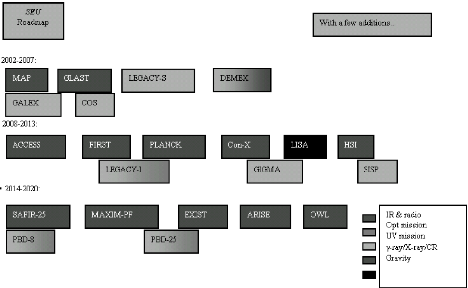
Figure 2 : The SEU roadmap with several UV-optical missions added. As in Figure 1, I use "SAFIR" to denote a large-aperture far-IR mission. The dates indicate approximate launch dates.
