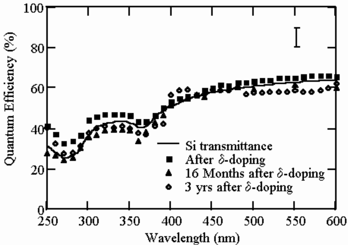
Figure 3. QE measured over a three-year period on the same delta-doped CCD. The CCD was stored unprotected in a laboratory environment. The error bars represent the accuracy ( \pm 5\% ) of the measurement systems used.
