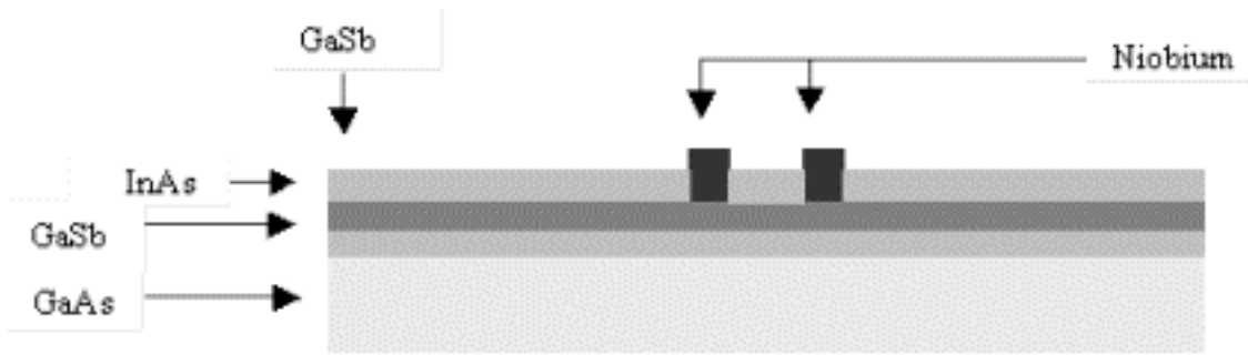
Figure 1: A Lateral Nb/InAs/Nb Structure
