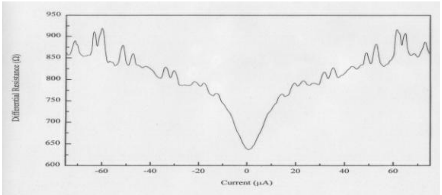
Figure 2: Differential Resistance Scans of a Superconducting Quantum Well taken at 350 mK
