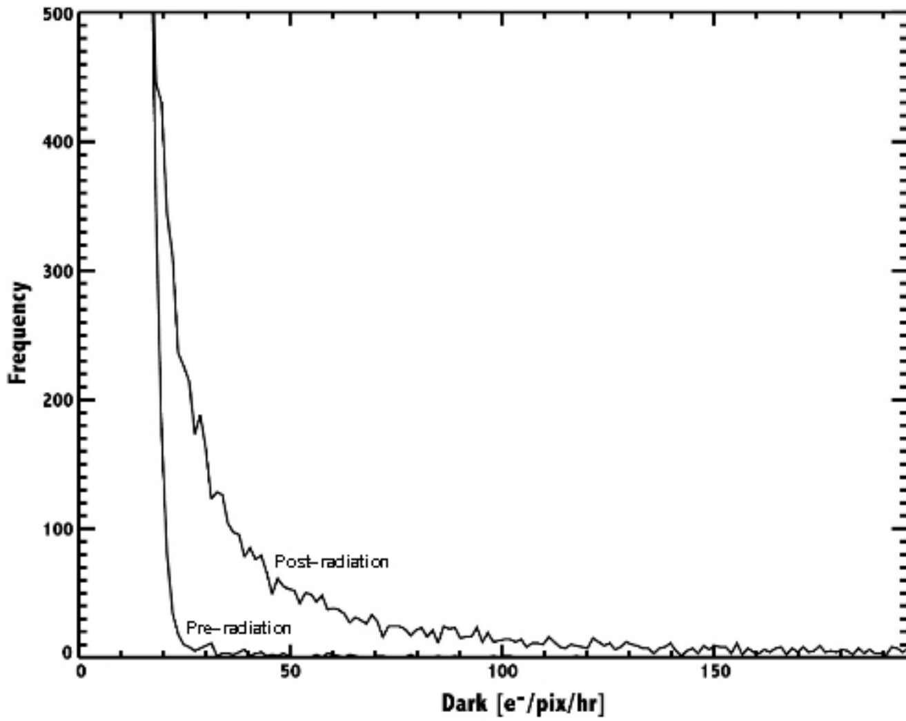
Figure 1. The tails of histograms of the dark signal for both pre- and post-radiation data. Note the expected increase in the size of the tail after irradiation.
