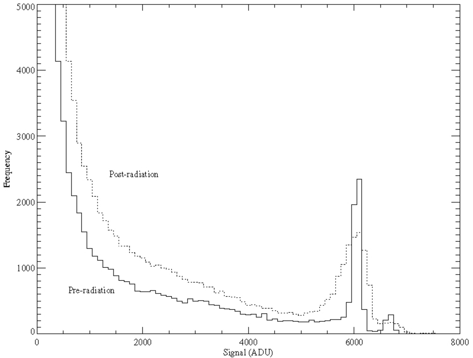
Figure 2. ^{55}\text{Fe} Signal Distribution for CCD44V1, pre- and post- radiation, channel A. Note how sharply defined K-alpha and are in the pre-radiation data(solid line). After irradiation (dashed line) K-alpha flattens and spreads and K-beta is not resolved.
