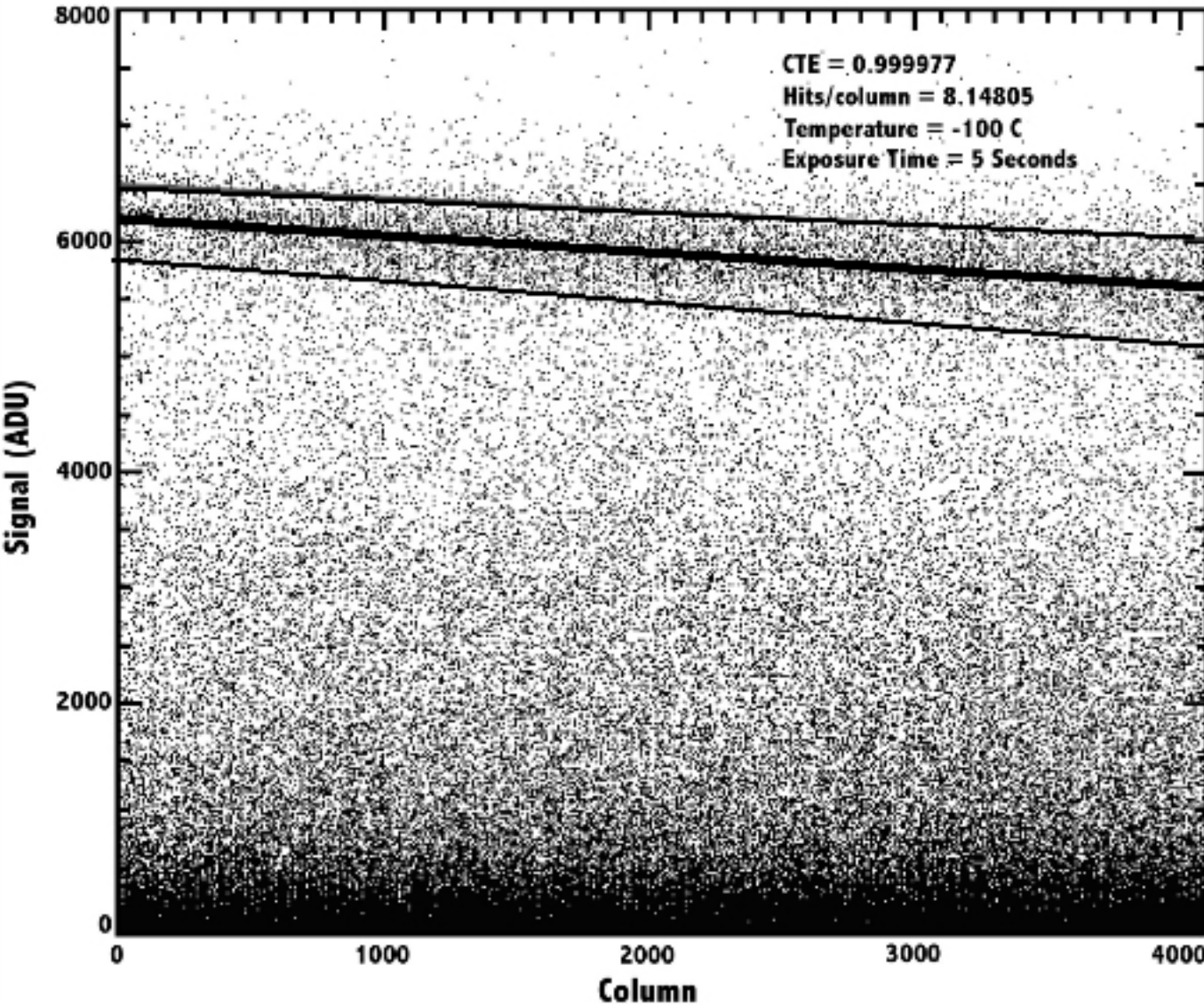
Figure 3. An example of a stacking plot of an ^{55}\text{Fe} image. The upper and lower lines denote the upper and lower bounds of K-beta our area of interest (the K-alpha line) and the middle line is the best fit to the area.
