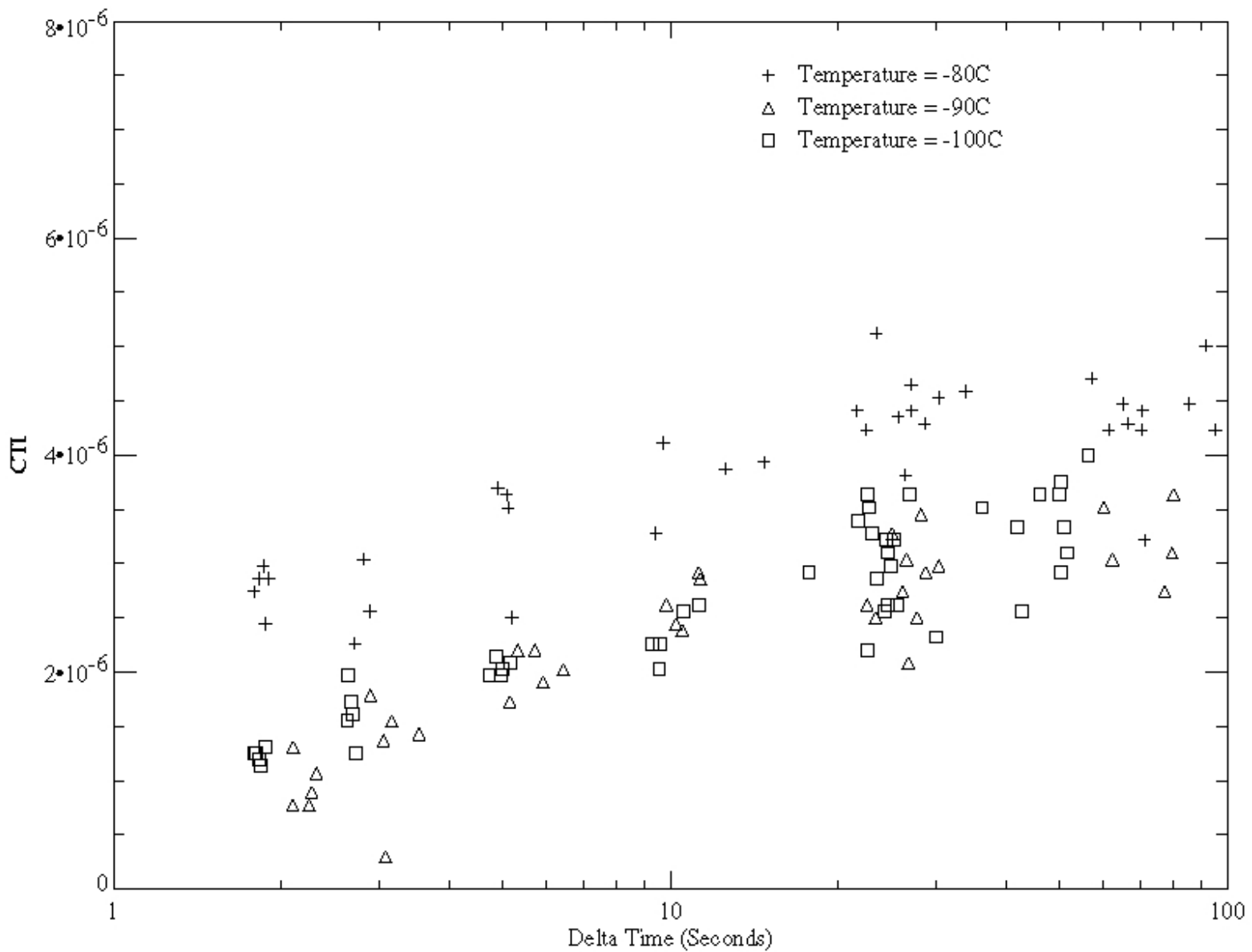
Figure 4. Charge transfer Inefficiency (CTI) vs Delta Time before irradiation. Note that data for -90C and -100C show no trend towards temperature dependence when CTI is good (pre-radiation). There is a marked improvement in CTI with an increase in signal.
