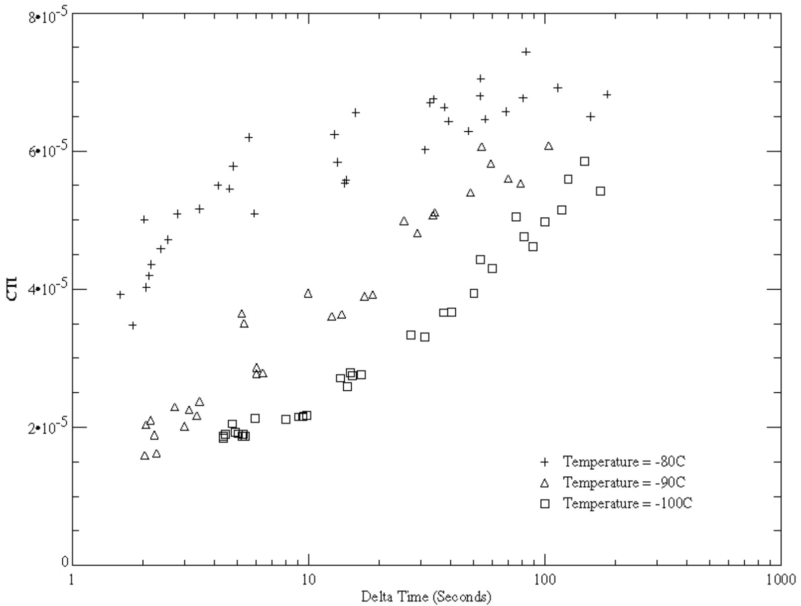
Figure 5. CTI vs Delta Time after irradiation. There is an obvious decrease in CTI with a decrease in temperature in addition to a strong trend to decrease CTI with an increase in signal density.
