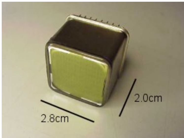
Figure 1 – Hamamatsu R5900-00-M64
