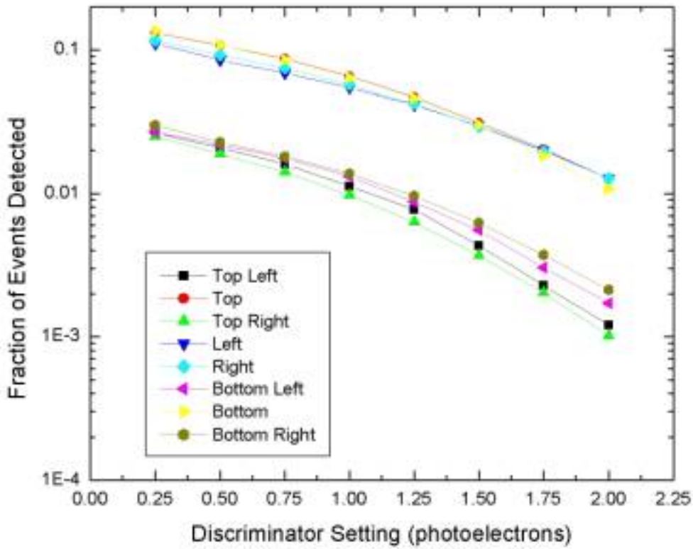
Figure 3 – Fraction of events detected in contiguous anodes around a 1 mm fiber centered on an anode versus discriminator setting
