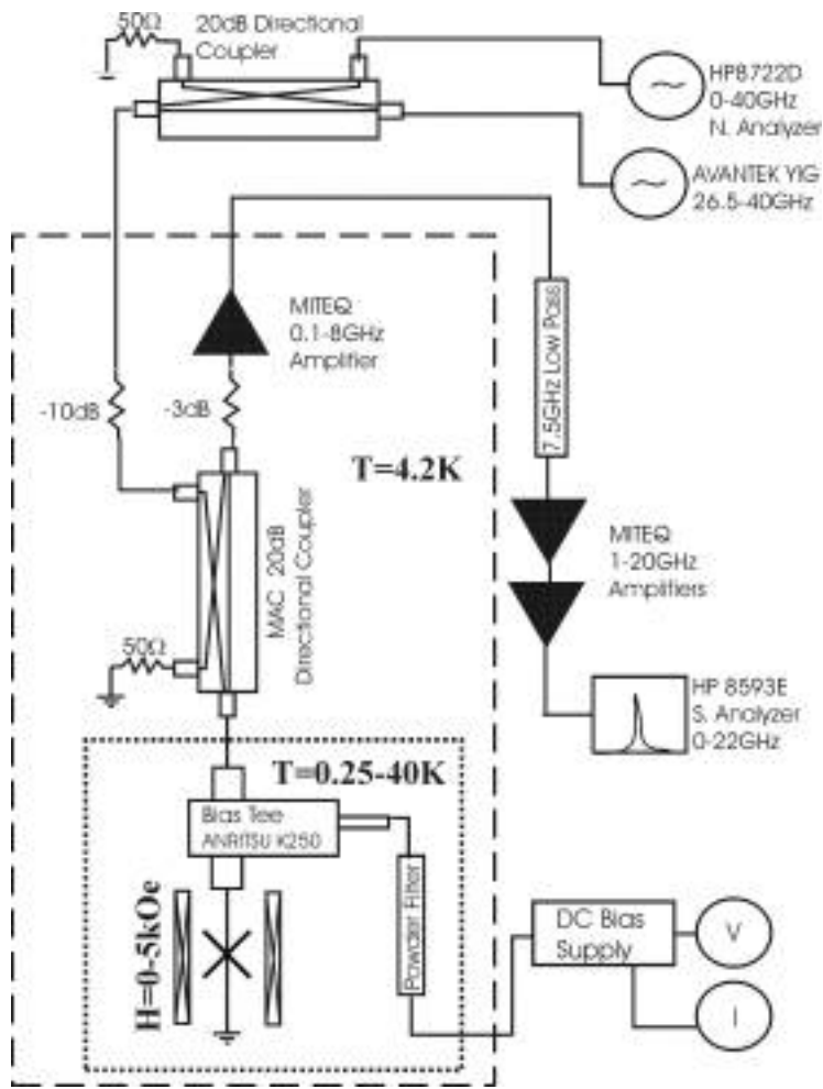
Fig. 1: Measurement Setup
