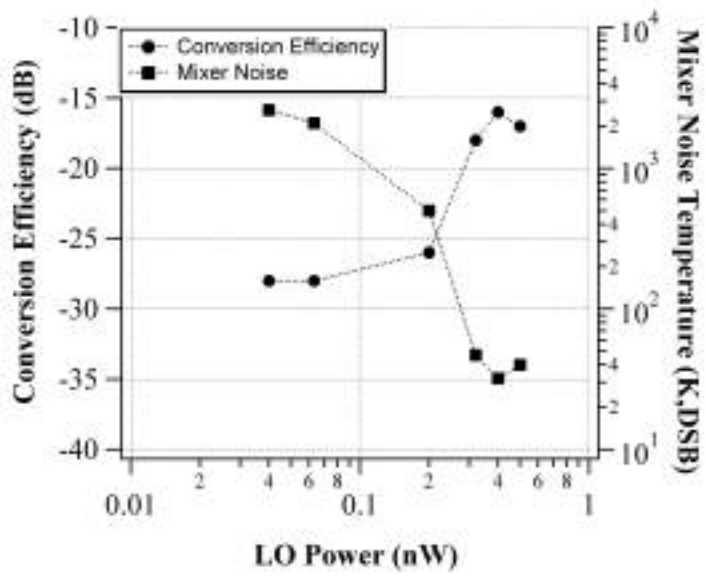
Fig. 3: Conversion Efficiency & Mixer Noise Temperature vs. LO Power. Device D. T=0.25K.
