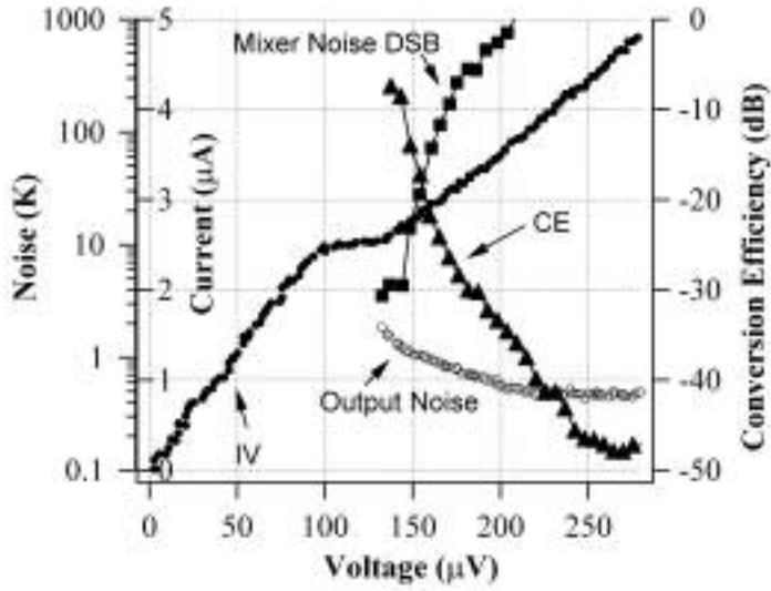
Fig. 4: Conversion Efficiency, Output Noise, and Mixer Noise vs. Bias Voltage for Device A. T=0.25\text{K} . H=1.2\text{kOe} .
