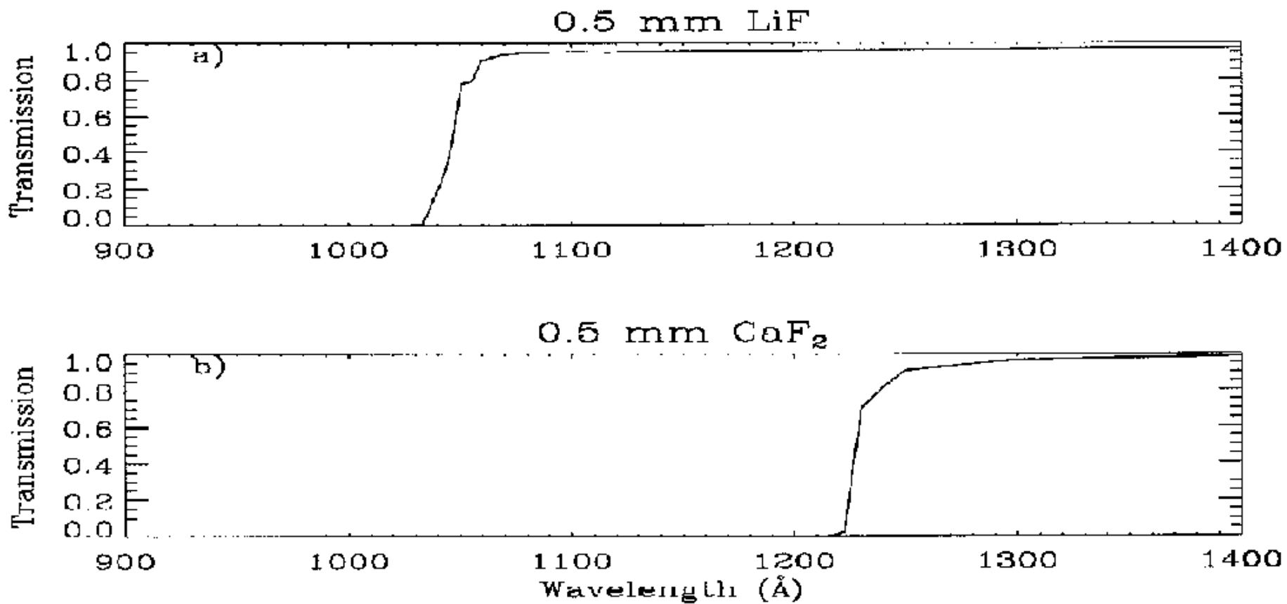
Figure 1. Transmission of a) 0.5 mm LiF, and b) 0.5 mm CaF 2 crystals.
