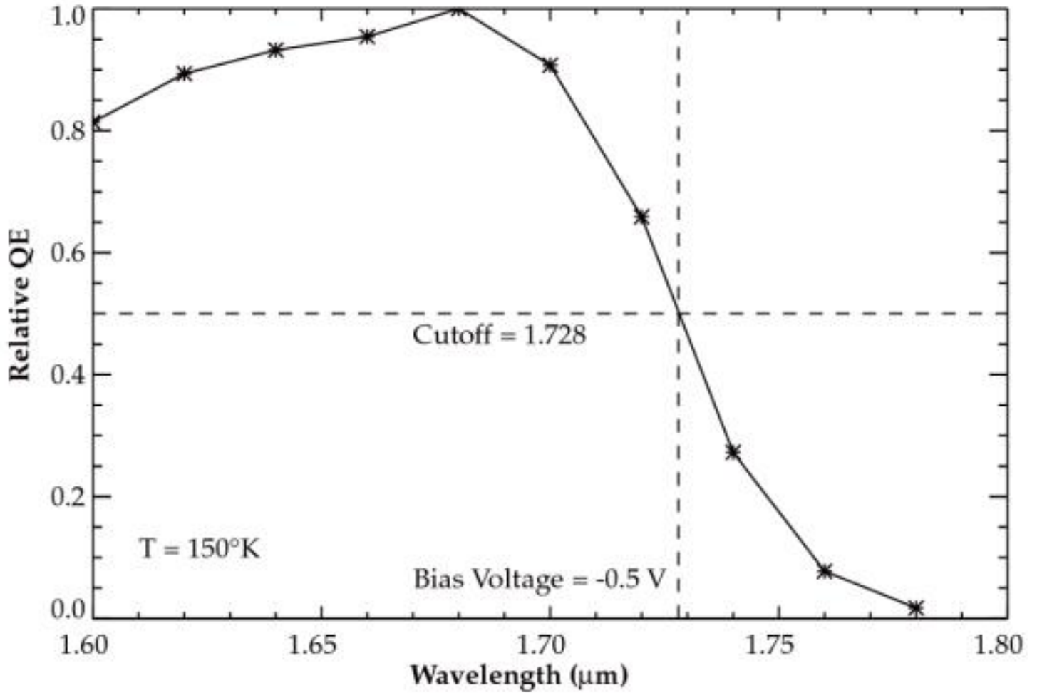
Figure 2 The relative quantum efficiency of the HgCdTe detector in the wavelength range near the long wavelength cutoff. The QE drops rapidly over a range of 0.1 \mu\text{m} from its maximum to near zero. The cutoff for this device is 1.73 \mu\text{m} .
