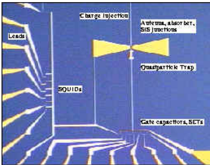
Figure 3: Optical picture of one field area of fabricated SQPC chip. The distance between two leads is 40 microns.
