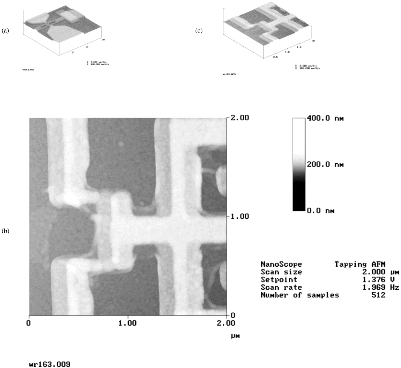
Figure 4: AFM images of (a) antenna, detector area, quasiparticle trap; (b) absorber strip, SIS junctions, SQUID loops; (c) SET
