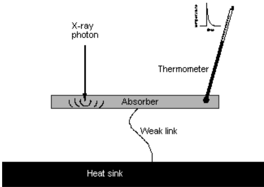
Figure 1 – Schematic of an x-ray calorimeter
