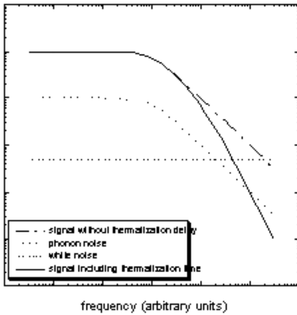
Figure 2 – Representative signal and noise spectra for a calorimeter. The units on the axes are arbitrary.
