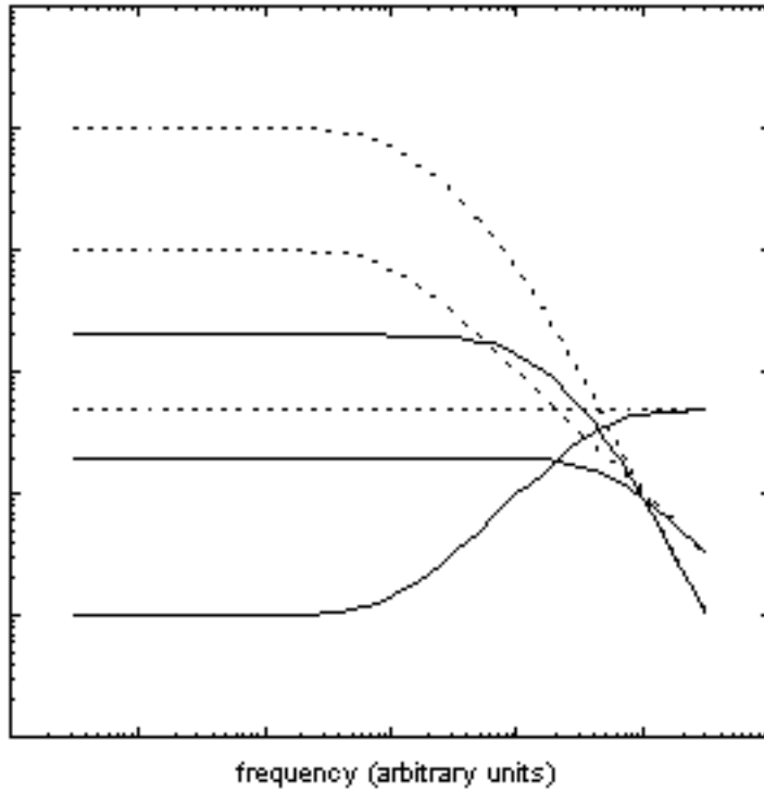
Figure 3 - Signal, phonon noise, and Johnson noise without electrothermal feedback (as in Figure 2 and shown in dashed lines) and with a large electrothermal feedback gain (shown in solid lines).
