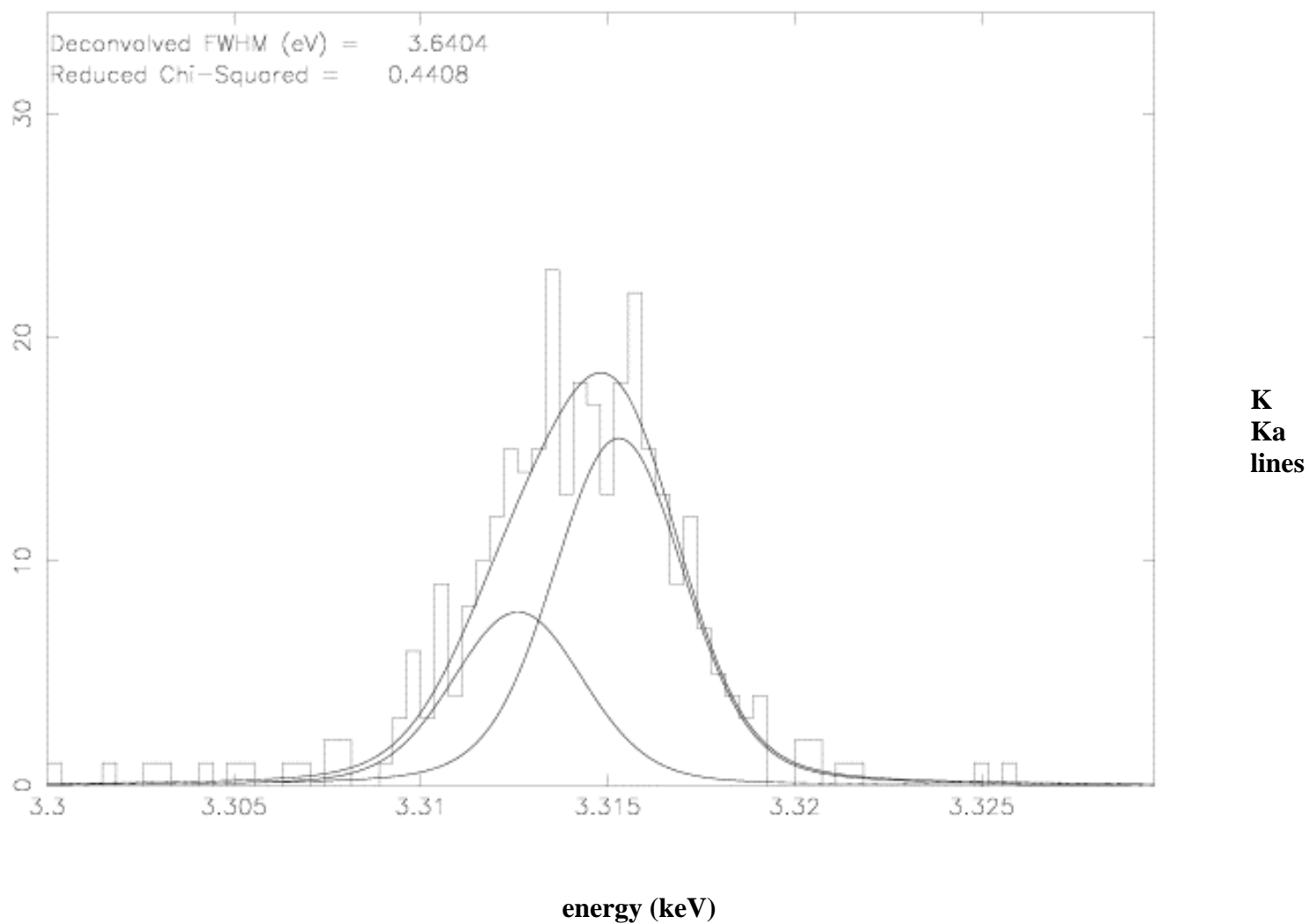
Figure 4 – 3.6 eV FWHM obtained with GSFC Mo/Au TES at 3.3 keV, the Ka_1 and Ka_2 lines of potassium.
