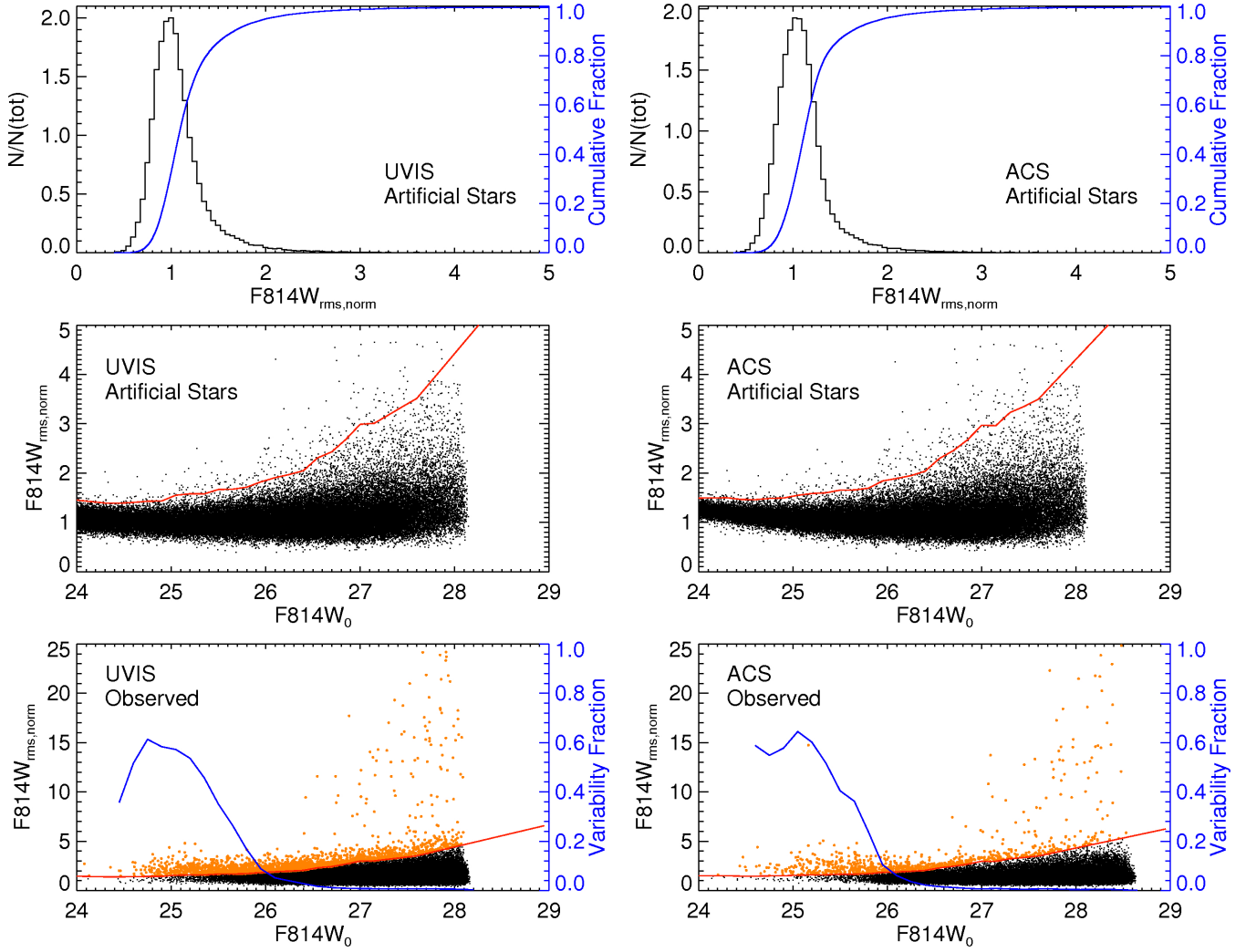
Figure 12. For the UVIS (left) and ACS (right) fields: Top: Histogram of F814W_{rms,norm} for input artificial stars which are assumed to be constant. The cumulative distribution of F814W_{rms,norm} is overplotted in blue with respect to the right-hand axis. Values shown here are after adding an additional per-epoch uncertainty of 0.025 mag (see text). Middle: Trend of F814W_{rms,norm} with F814W magnitude for the artificial stars. Our criterion for defining variables from the 99.5% observed envelope is overplotted in red. Bottom: F814W_{rms,norm} versus mean F814W for observed stars, with our variability criterion overplotted and candidate variables shown in orange (note the difference in y-axis scale compared with the middle panel). The variability fraction is overplotted in blue with respect to the right-hand axis.
