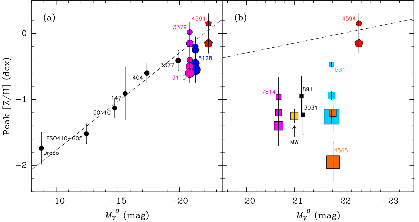
Figure 9. Peak [Z/H] of the MDF of RGB stars in halo fields around nearby galaxies as function of galaxy M_V^0 (see Table 3). Panel (a): data for early-type galaxies (ETGs). Labels next to data points indicate the NGC number of the galaxy in question (unless indicated otherwise). Small black circles indicate ETG fields with R_{\text{gal}}/R_{\text{eff}} \leq 5 , and the dashed line represents a linear least-squares fit to those data. Symbols and labels with colors other than black represent galaxies with more than one field, and the sizes of those symbols scale with R_{\text{gal}}/R_{\text{eff}} of the field in question. Our two halo fields in the Sombrero are represented by red pentagons. Panel (b): Similar to panel (a), but now showing data for luminous spiral galaxies. Note the different range in M_V^0 . Small black squares indicate halo fields in spirals for which the dependence of peak [Z/H] on R_{\text{gal}} is negligible according to Monachesi et al. (2016). The Milky Way (MW) halo is represented by a yellow square. The dashed line is the same one as in panel (a).
