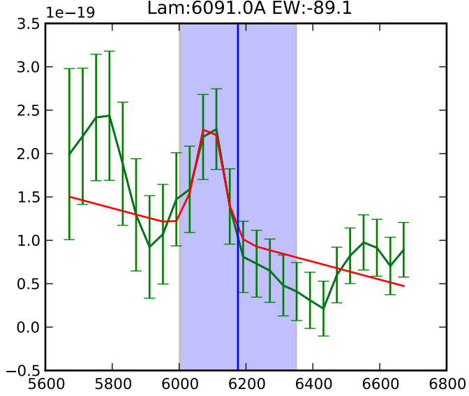
PA:116 flux:1.3e-17 F: 38.6A Lam:6091.0A EW:-89.1
