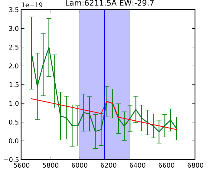
PA:066 flux:8.2e-18 F: 9.3A Lam:6211.5A EW:-29.7
