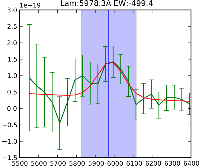
PA:112 flux:1.9e-17 F: 68.6A Lam:5978.3A EW:-499.4
