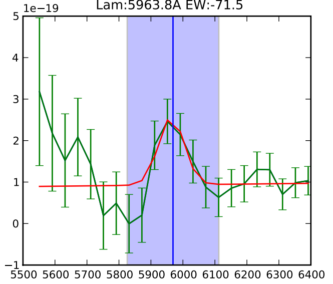
PA:080 flux:1.6e-17 F: 39.7A Lam:5963.8A EW:-71.5
